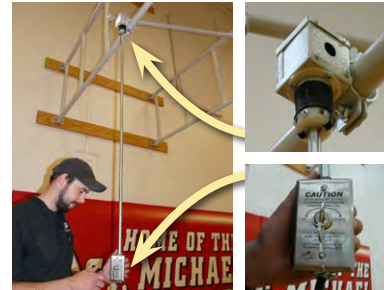
Portable Electric Wand Operation (BA980EW)
