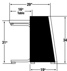
All Convertible Tables on Floor
