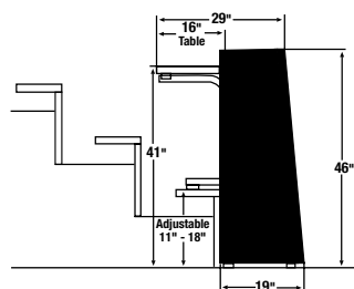
All Space Saver Tables
