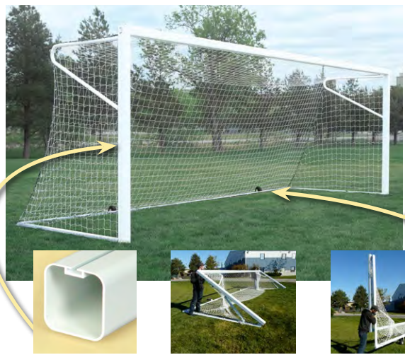
4" Square Large Corner Safety Radii Support goal as it is lowered. Roll on 12" semi-pneumatic swivel casters.
