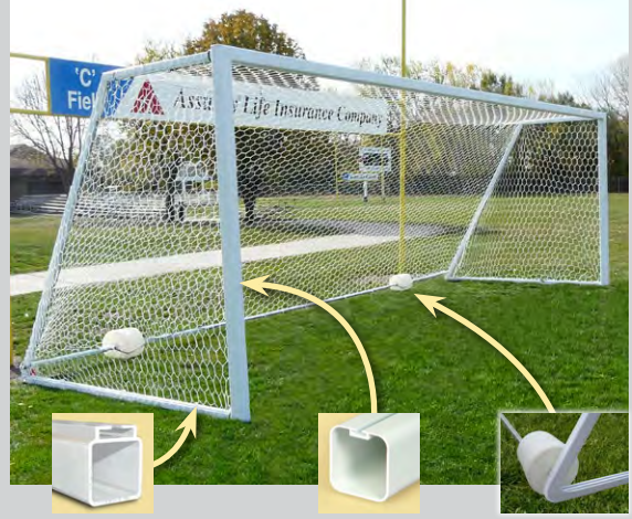
2" Square QwikTrack™ Side and Rear Rails 4" Square Large Corner Safety Radius No-Tip Transport/Ballast System
