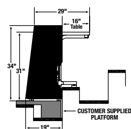
All Convertible Tables in Bleachers
